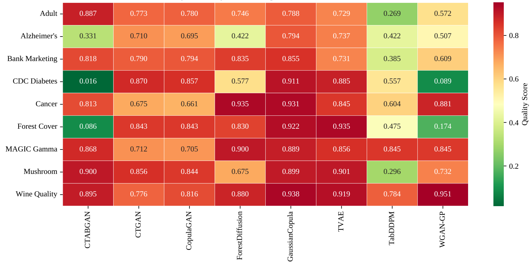
Quality Score by dataset × generator (10-seed mean)
